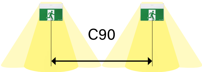
MAXIMUM SPACING FOR 1 LUX (NEW ZEALAND)
